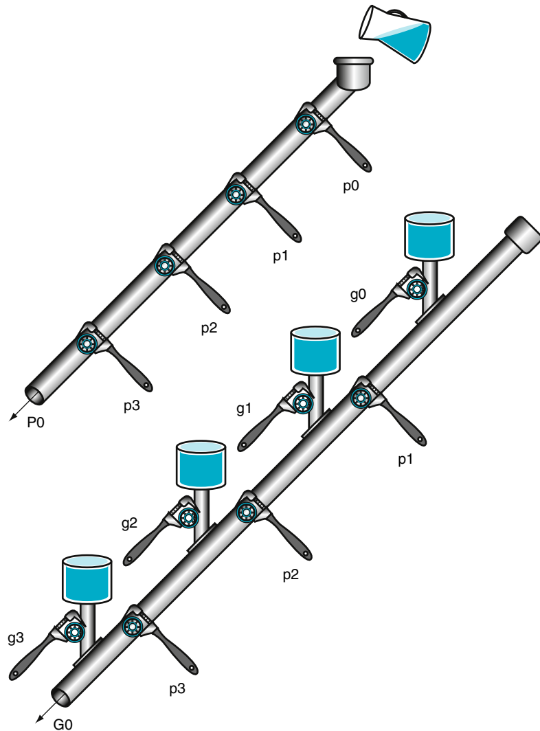
FIGURE A.6.2 A plumbing analogy for the next-level carry-lookahead signals P0 and G0 . P0 is open only if all four propagates ( p_i ) are open, while water flows in G0 only if at least one generate ( g_i ) is open and all the propagates downstream from that generate are open.
